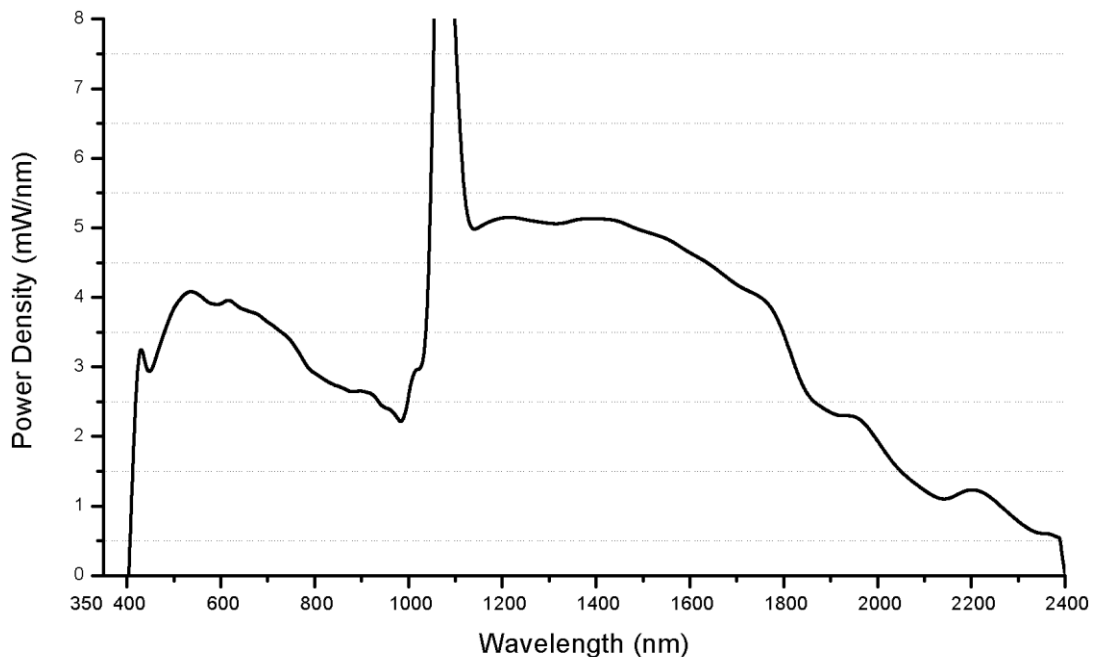
8W SC Pro Typical Spectrum (4MHz)
